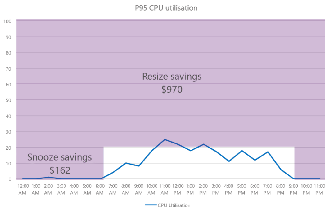
Figure 5-4 CPU utilisation of IaaS app
